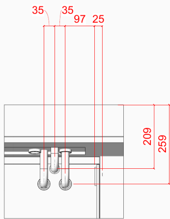
9 3D - W57_Lucht Detail CV/Condens
